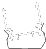
FIXING CLIP 15°
