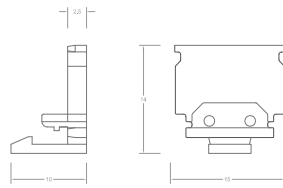
IN CAP (transparent)
