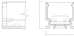
PROFILE + CAP (SIDE VIEW)
